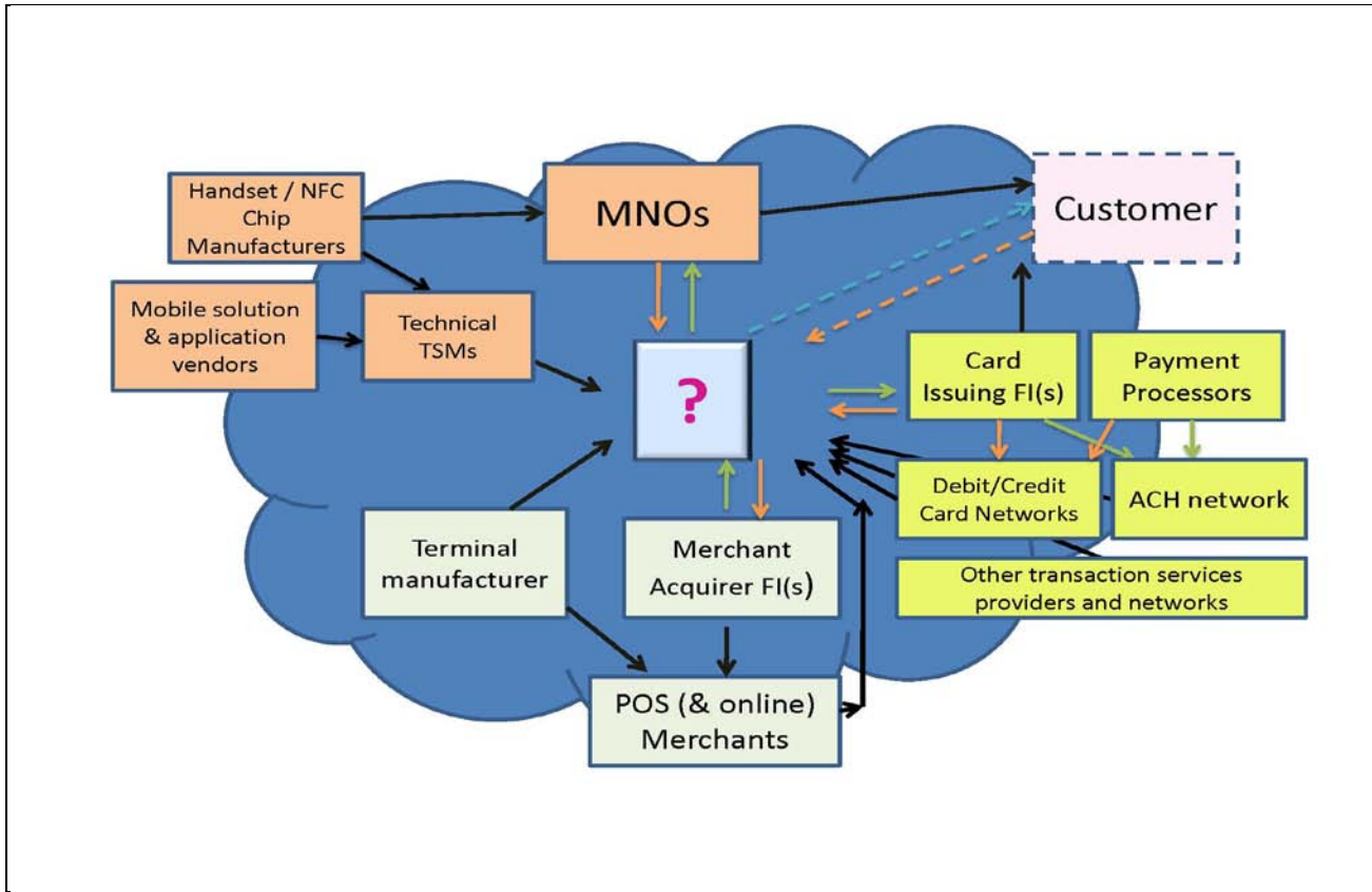
Figure 1: Collaborative Model
